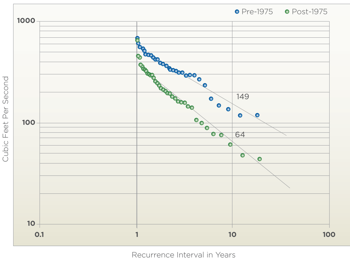
Figure 2-1: Seven-Day Minimum Flows— Flint River at Carsonville Gauge, 1940-2011
