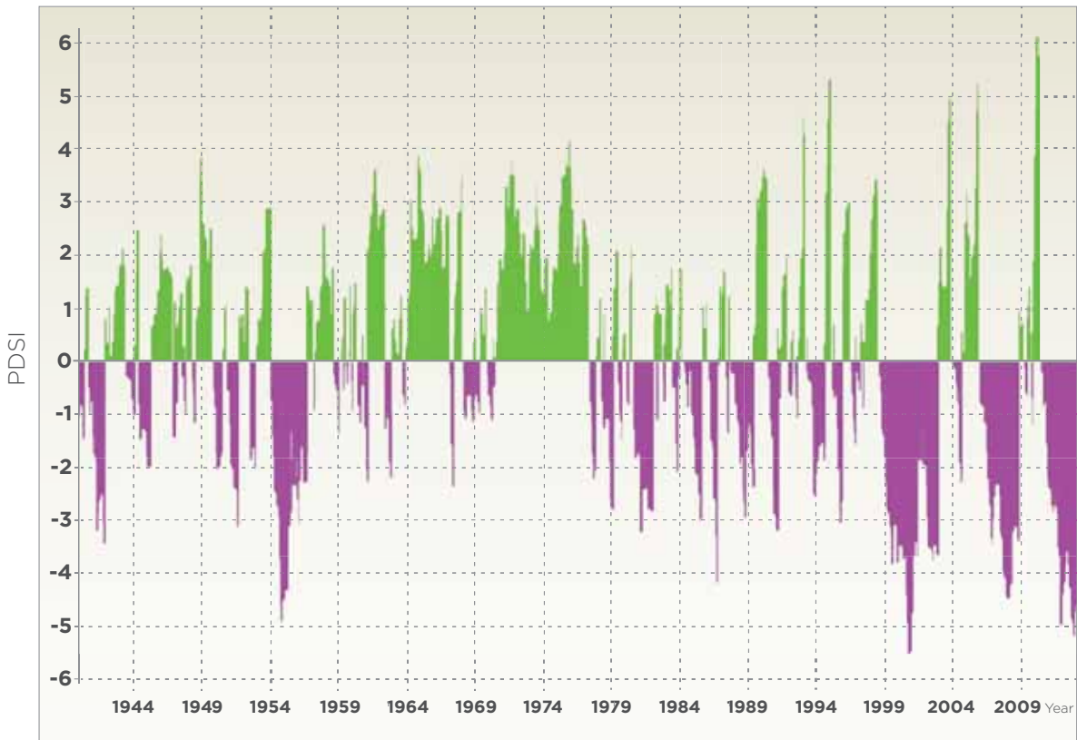
Figure A-3: Palmer Drought Severity Index—West-Central Georgia, 1940-2012
